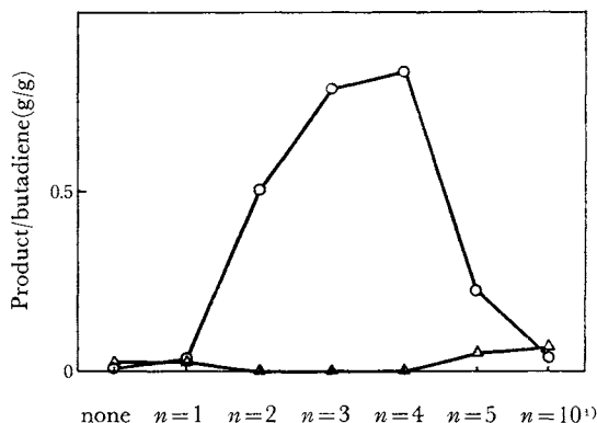
Fig. 1. Effect of the length of methylene chain in catalyst of \text{CoCl}_2(\text{Ph}_2\text{P}(\text{CH}_2)_n\text{PPh}_2)\text{-AlEt}_3 reaction condition: see footnote a) in Table 1, \text{Al/Co}=8-10
